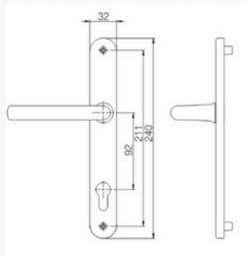
MILA PROSTYLE OVAL LEVER HANDLE 240MM
