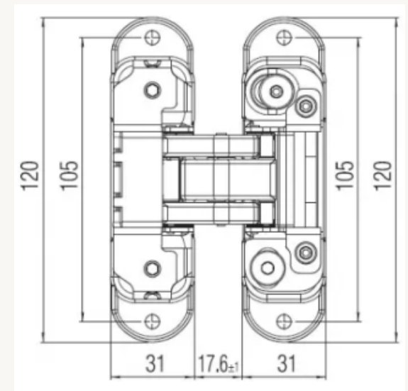
CONCEALED HINGES - ATOMICA
