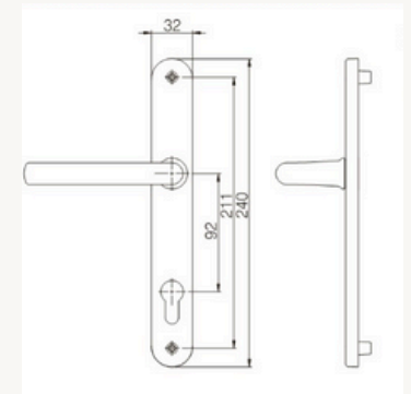
MILA PROSTYLE SWEEP LEVER HANDLE 240 MM
