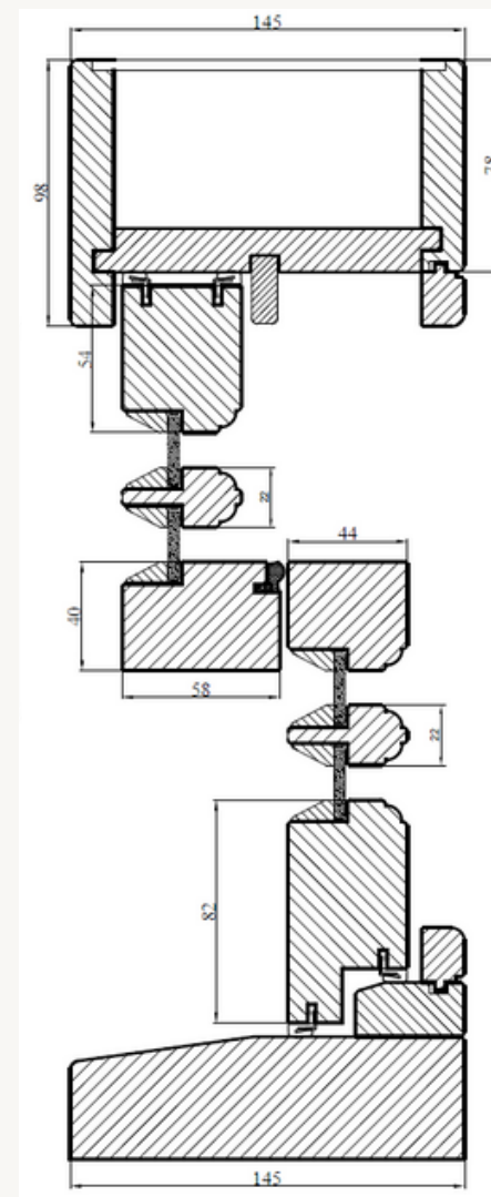
SLIDING SASH 145/44 WITH PUTTY IMITATION
