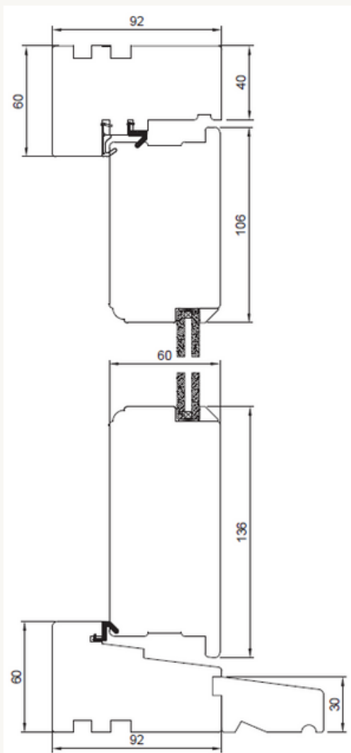
CASEMENT SD WITH PUTTY IMITATION
