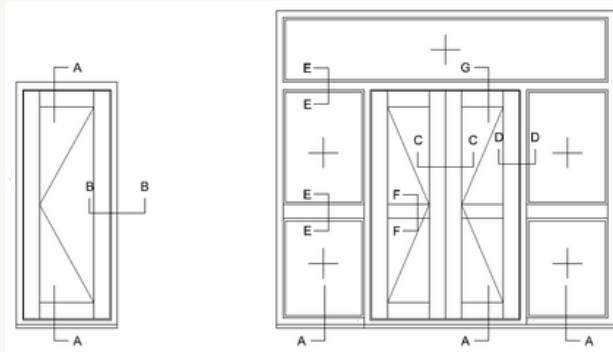
FLUSH DOOR SD IN - FRAME OVOLO/ SQUARE
