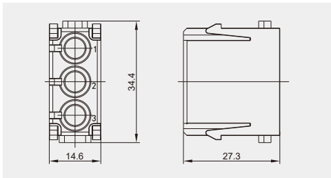
Dimension and hole site
