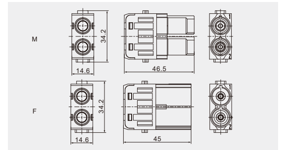
Dimension and hole site
