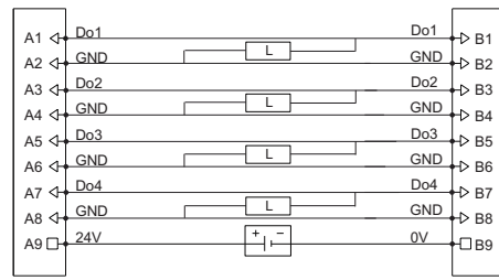
Wiring Diagram
