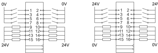
DF20-M-8DIO-N
