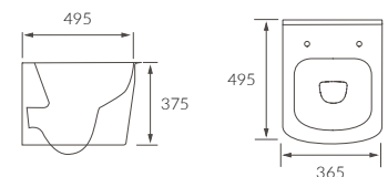
RIMLESS WALL HUNG PAN SHORT PROJECTION
