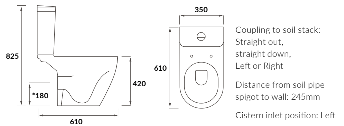
SWIRLUX CLOSE COUPLED SHORT PROJECTION PAN AND CISTERN OPEN BACK
