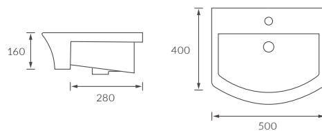
SEMI RECESSED BASIN
