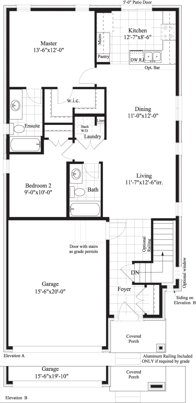
First Floor
