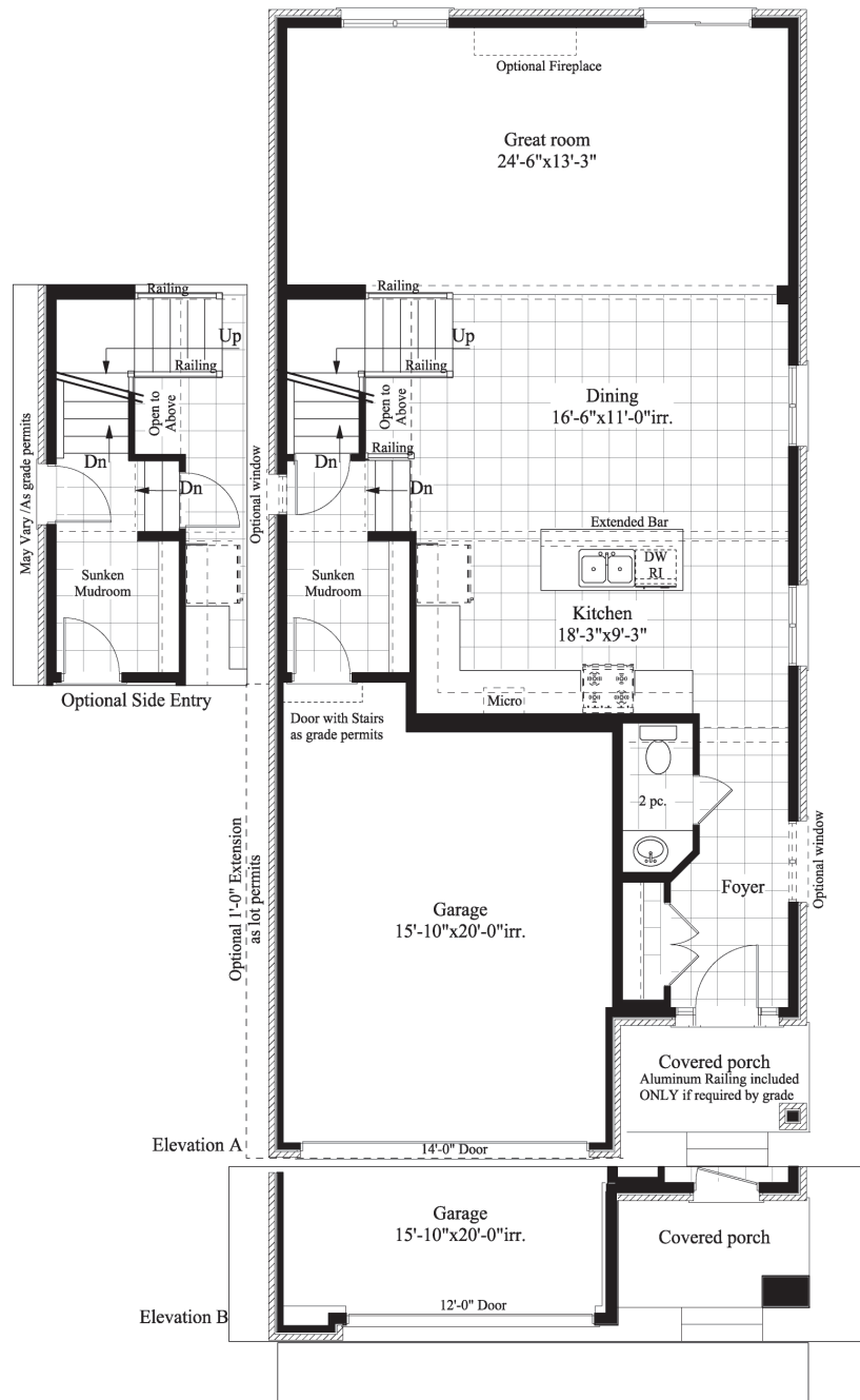
First Floor
