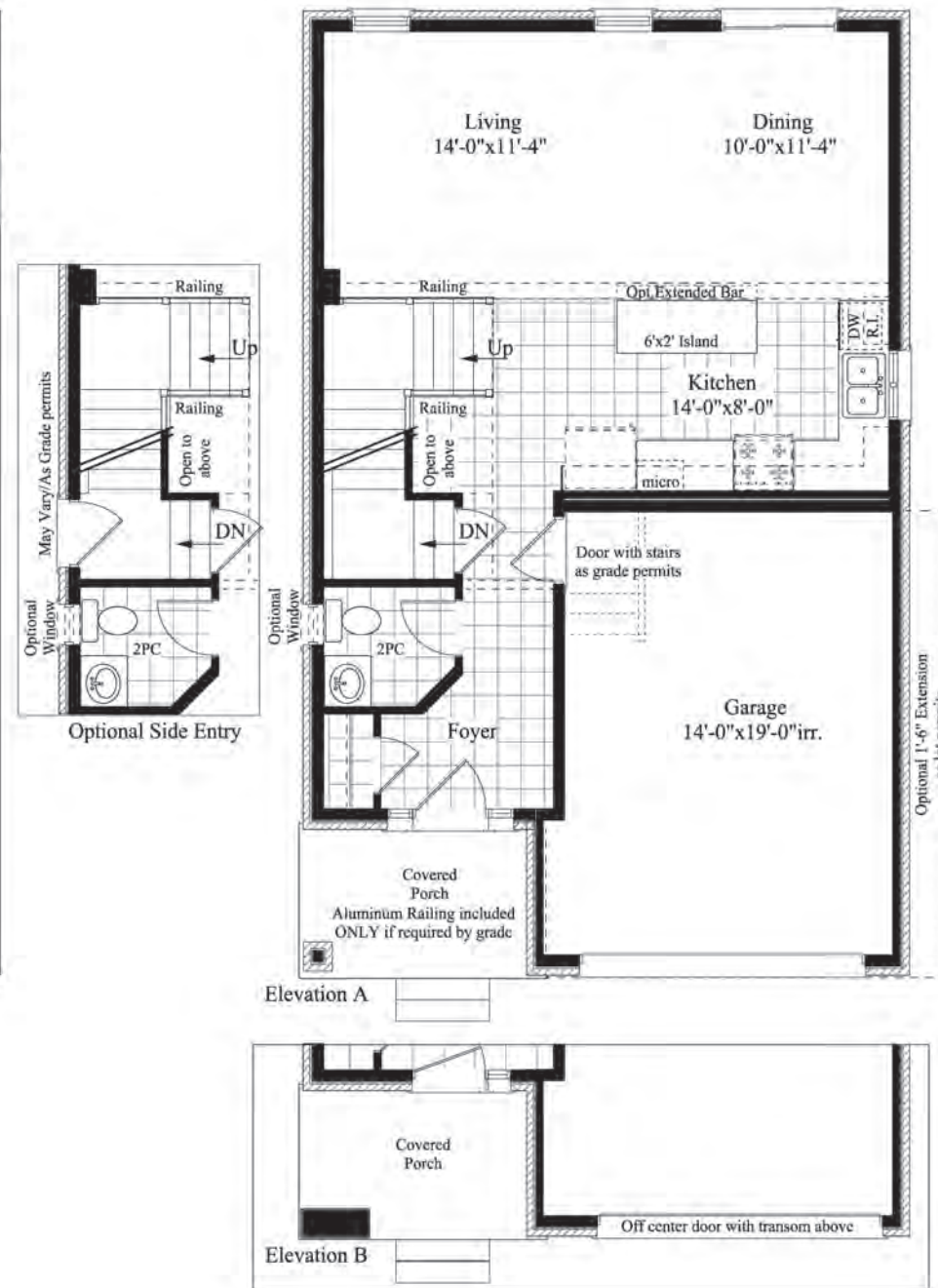
First Floor
