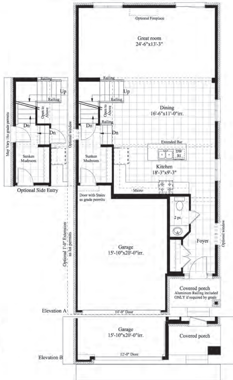
First Floor
