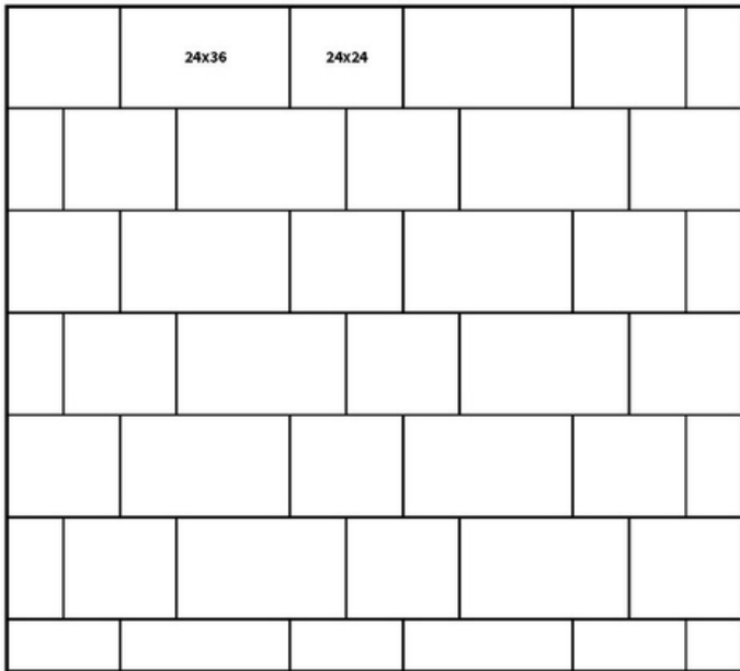
24"x 24"&24"x 36" Alt. Running Bond 40sf 24"x24" 60sf 24"x36"
