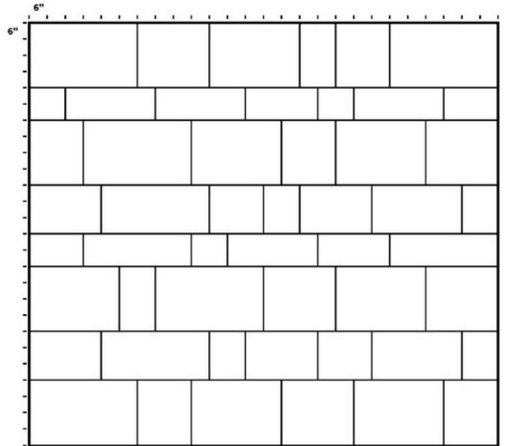
Mixed Height Random Running Bond (12", 18", and 24" Height in Mixed Lengths)
