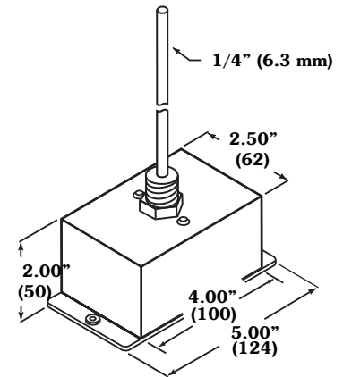
Figure 3: IMMERSION ENCLOSURE
