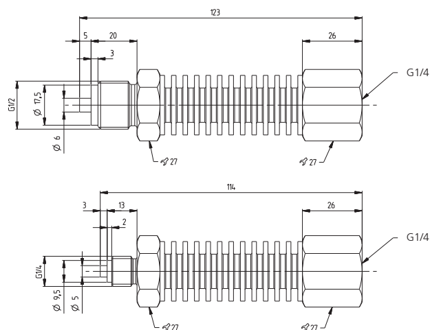
Heat sink
