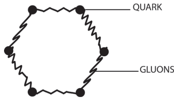
The atoms subatomic structure strong force of nature gluons and quarks.
